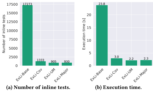
Figure 9: Number and execution time of inline tests extracted by ExLi with different levels of reduction.
